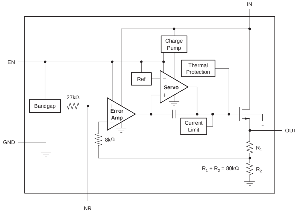
Figure 2. Fixed Voltage Version
